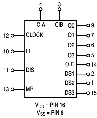
Figure 1. Block Diagram
